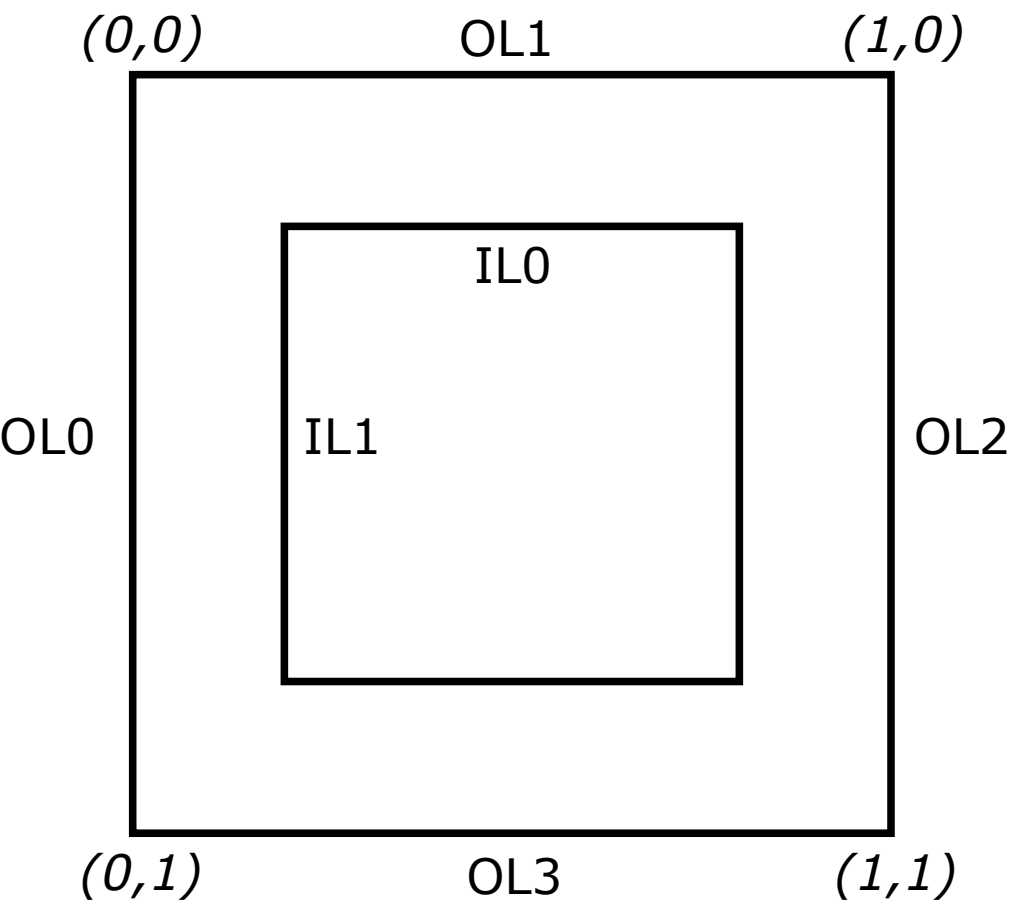
Quads
