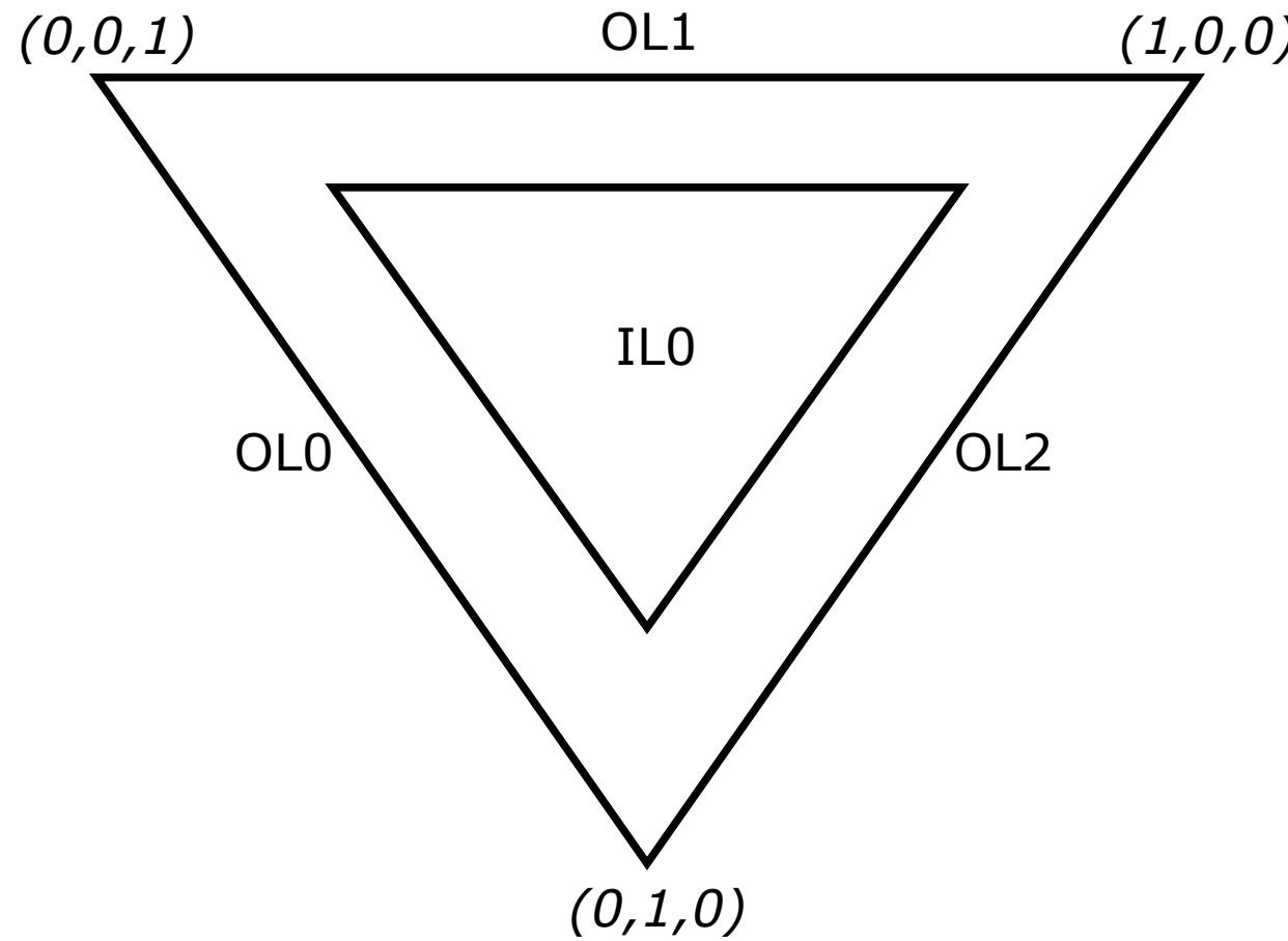
Triangles
