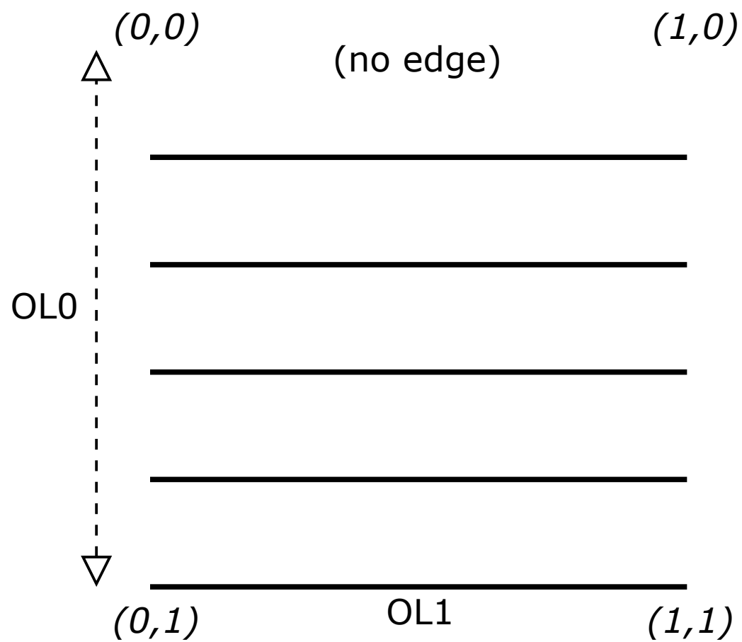
Isolines
